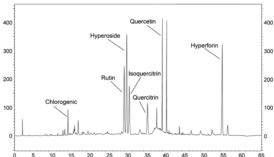
FIG. 3. St. John's wort ( Hypericum perforatum ) HPLC chromatogram.
